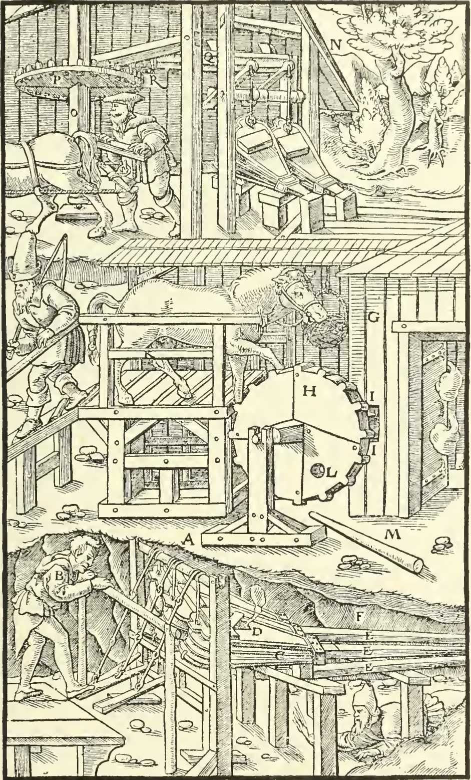
A—MACHINE FIRST DESCRIBED. B—THIS WORKMAN, TREADING WITH HIS FEET, IS COMPRESSING THE BELLOWS. C—BELLOWS WITHOUT NOZZLES. D—HOLE BY WHICH HEAVY VAPOURS OR BLASTS ARE BLOWN OUT. E—CONDUITS. F—TUNNEL. G—SECOND MACHINE DESCRIBED. H—WOODEN WHEEL. I—ITS STEPS. K—BARS. L—HOLE IN SAME WHEEL. M—POLE. N—THIRD MACHINE DESCRIBED. O—UPRIGHT AXLE. P—ITS TOOTHED DRUM. Q—HORIZONTAL AXLE. R—ITS DRUM WHICH IS MADE OF RUNDLES.
